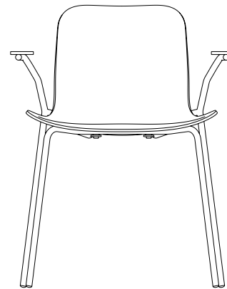
LANGUE CHAIR W/ ARMREST W 57 CM | D 51 CM | H 78 CM SH 46 CM | SH w/ Upholstery 47 CM Armrest Height 67,5 CM
